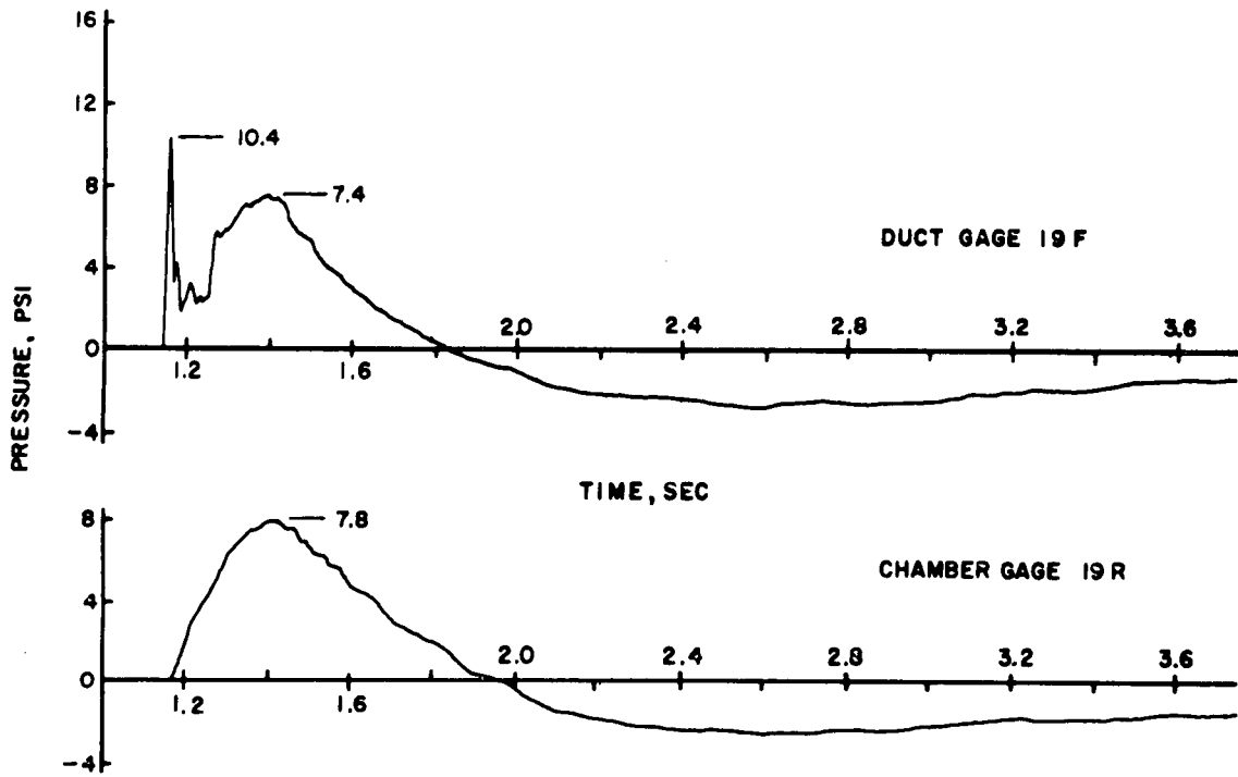
Fig. 7—Pressure-time curves for T-shaped vent, shot 9.
